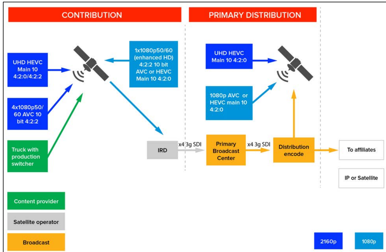
Figure 7 Contribution Workflow
