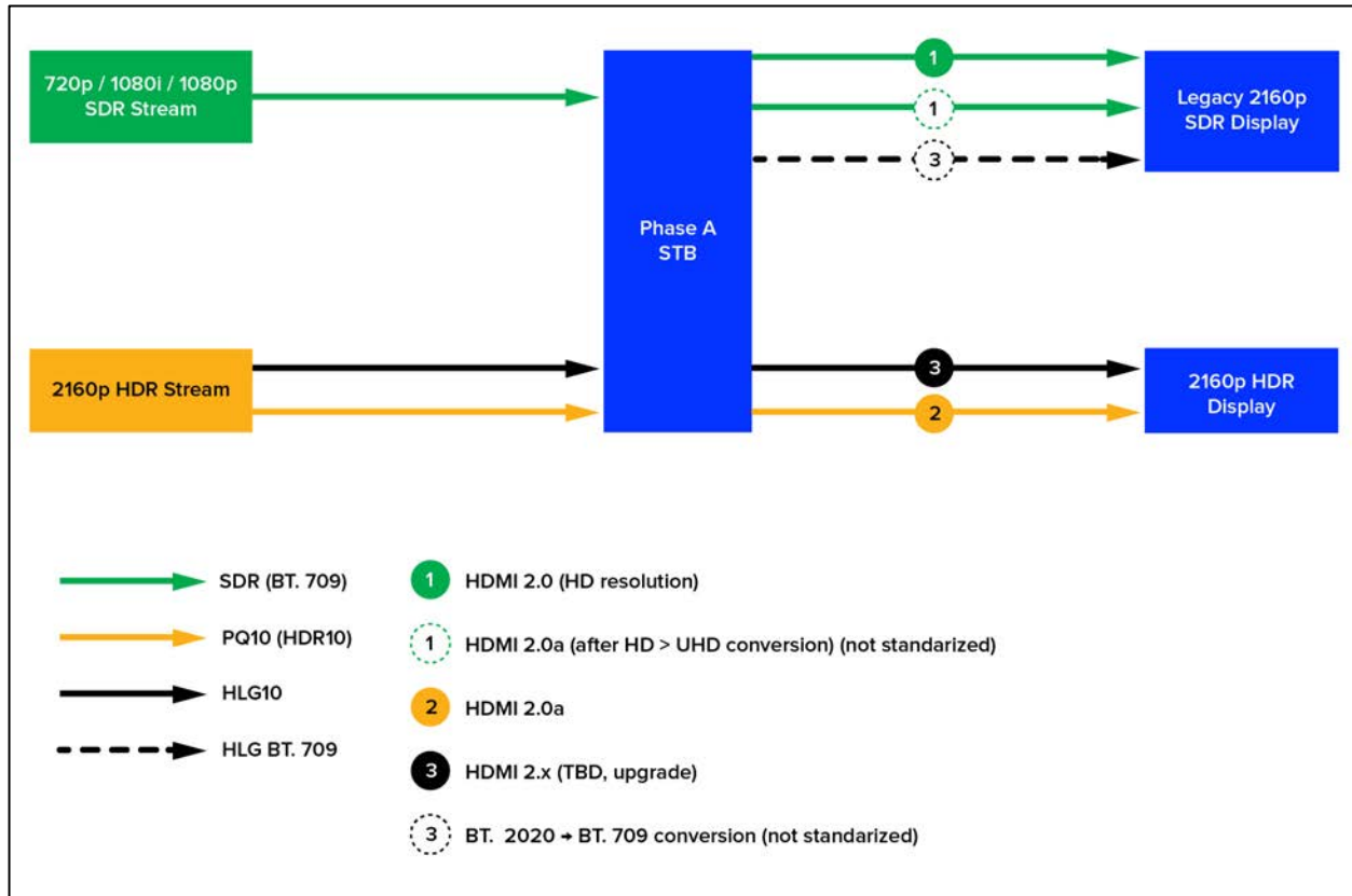
Figure 12 Spatial Resolution Up-conversion of Legacy Services
