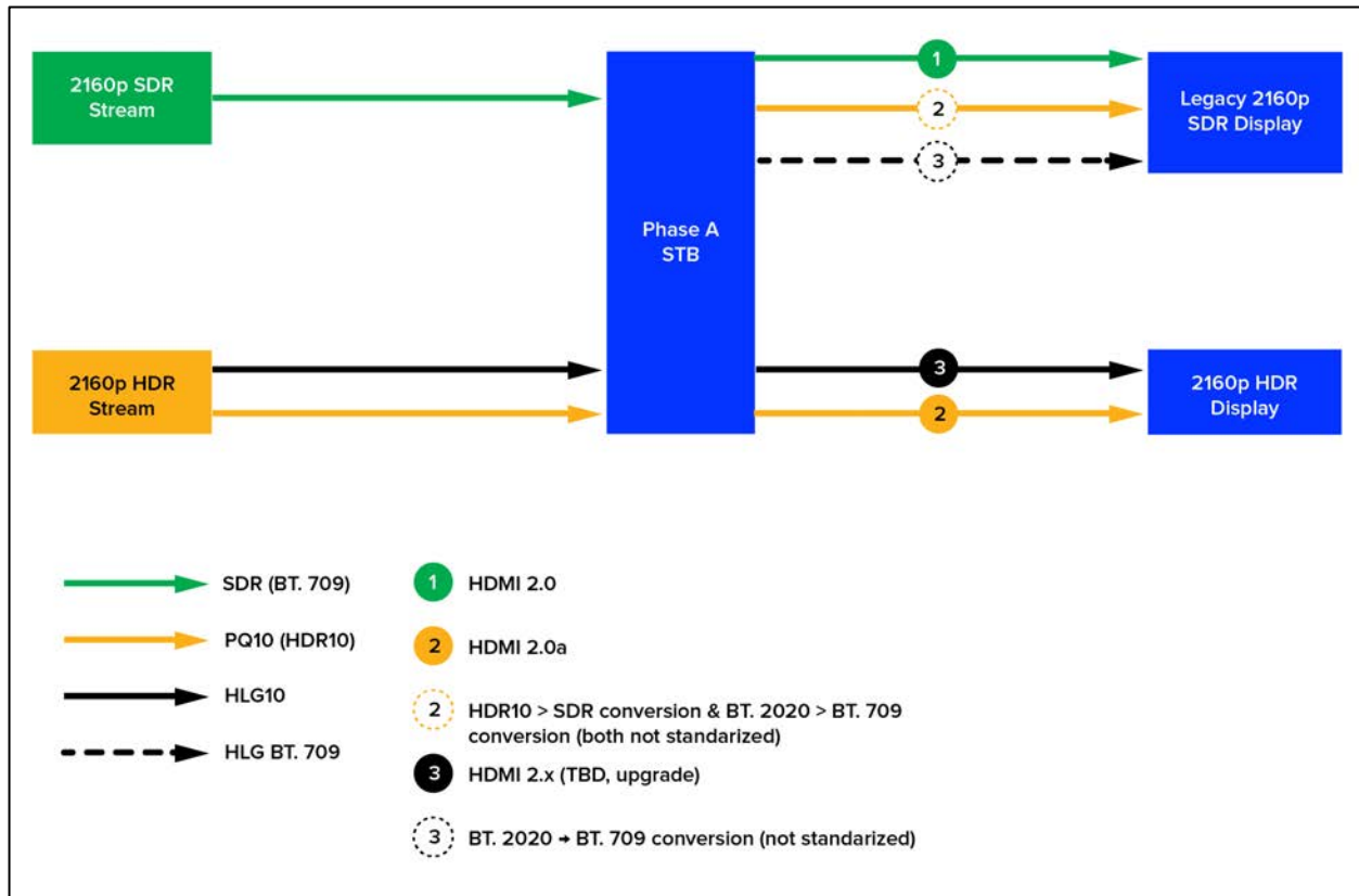
Figure 11 Down-conversion at the STB
