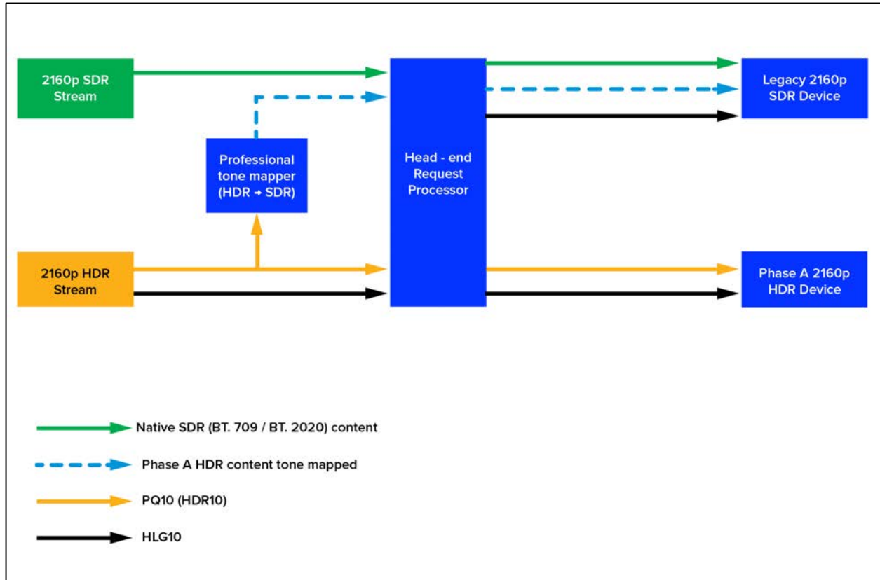
Figure 10 Down-conversion at the Headend
