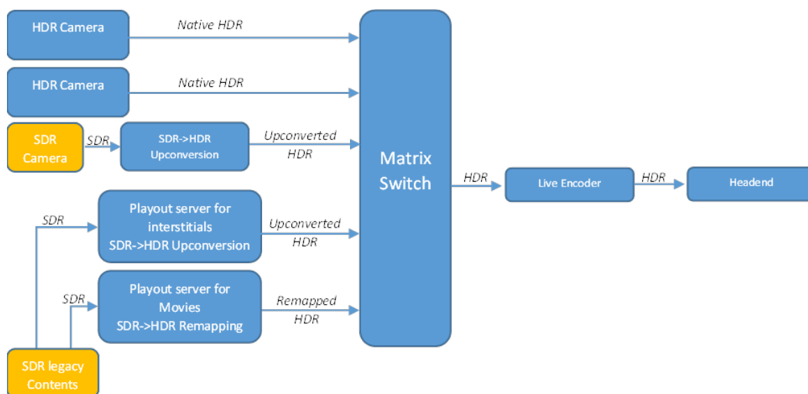
Figure 5 Sample Live Workflow with Mixed Format Source Content
