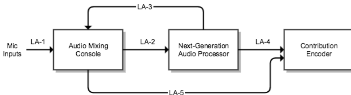
Figure 4 Channel-based Immersive Audio Live Production
