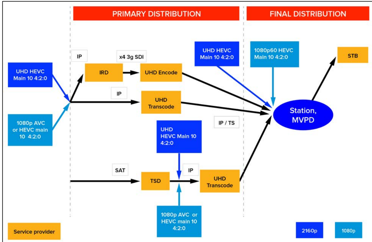
Figure 8 Primary Distribution to an MVPD or Station
