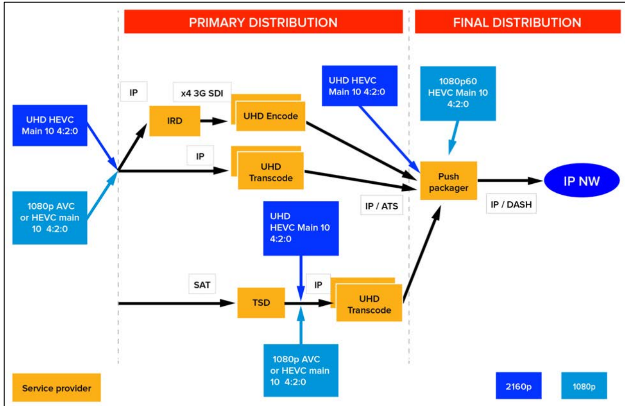
Figure 9 Primary Distribution to an OTT Provider
