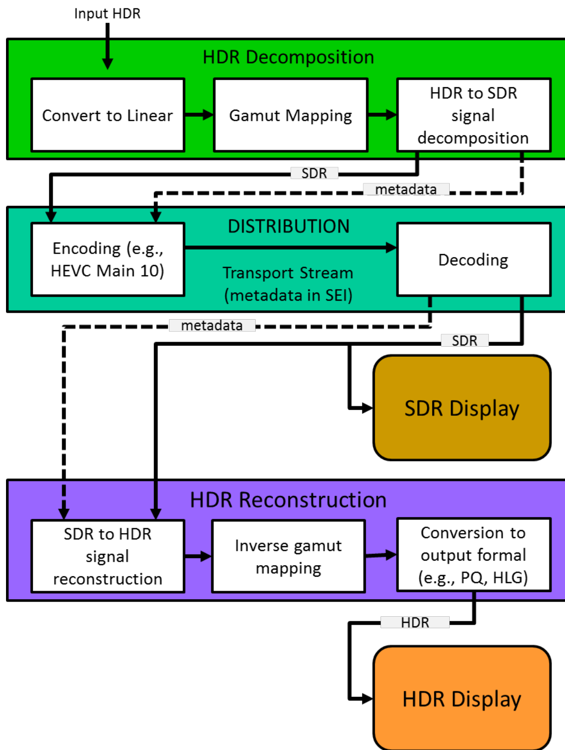
Figure 16 Phase B SL-HDR1 Processing, Distribution, Reconstruction, and Presentation
