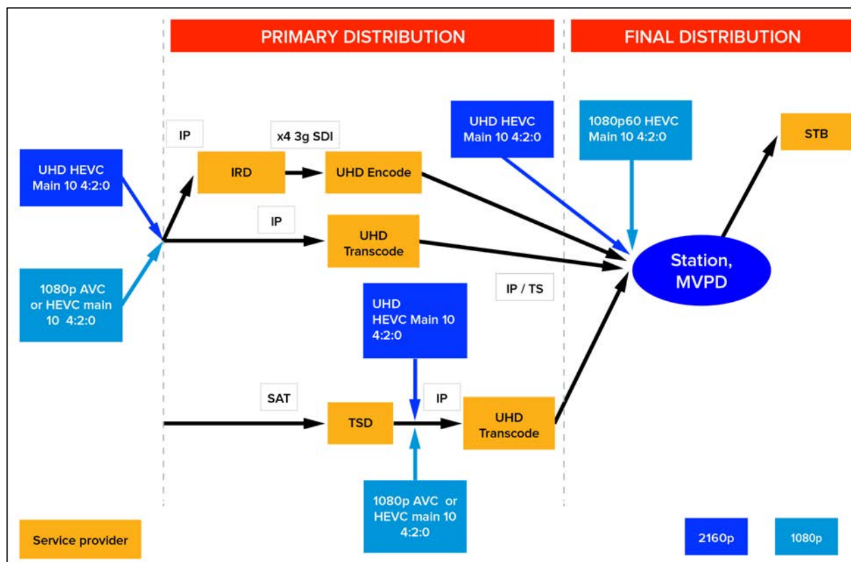
Figure 8 Primary Distribution to an MVPD or Station
