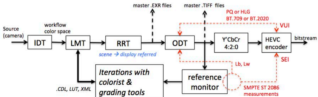
Figure 15 ACES Workflow Model
