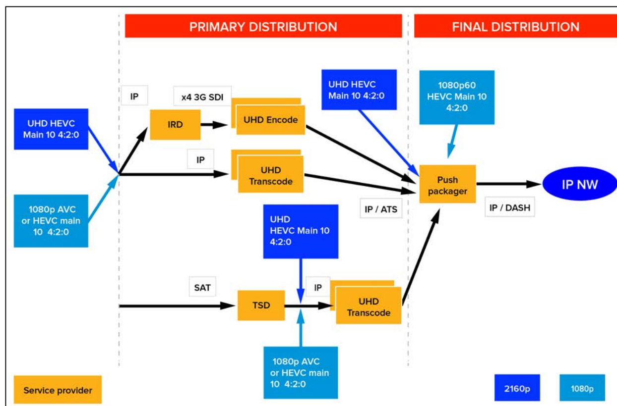
Figure 9 Primary Distribution to an OTT Provider
