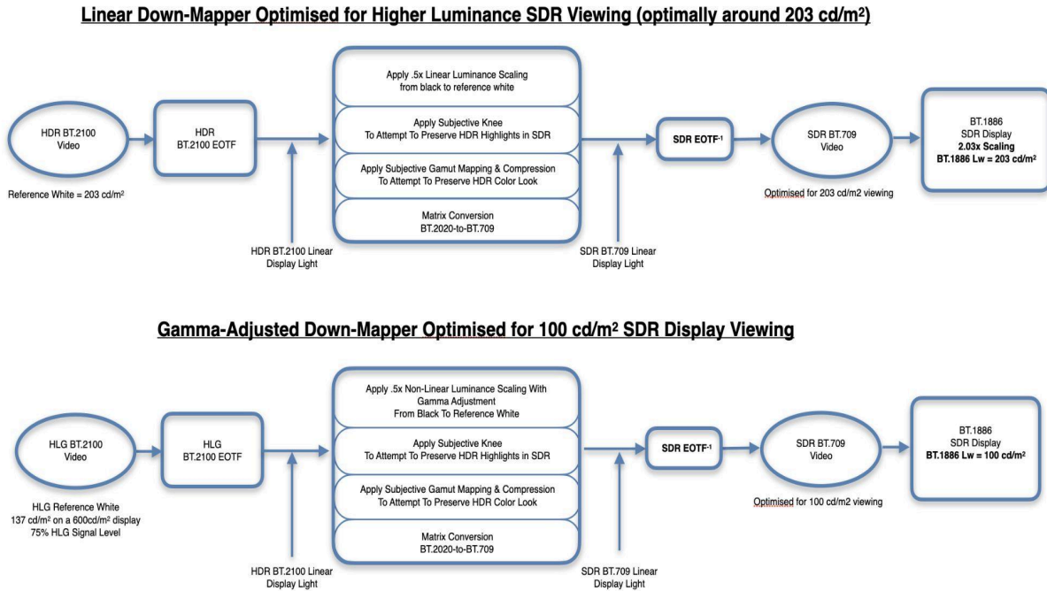
Figure 5: Two Conversion Workflows Through HDR to SDR Down-mapping
