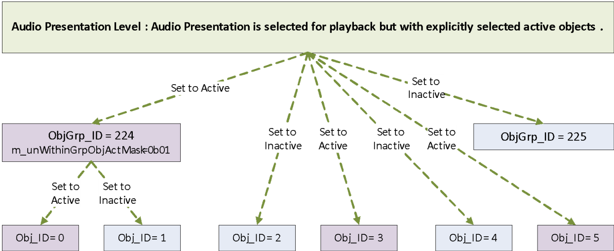
Figure 31. Specific Object and Group Selection
