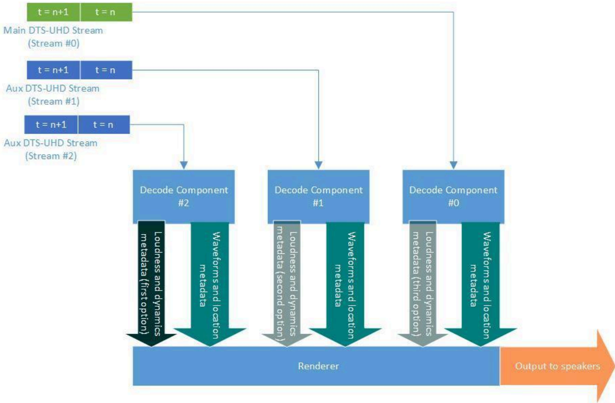
Figure 35. Example of multi-stream decoding
