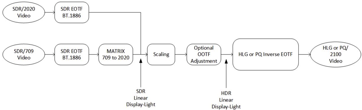
Figure 86. Display Light Conversion
