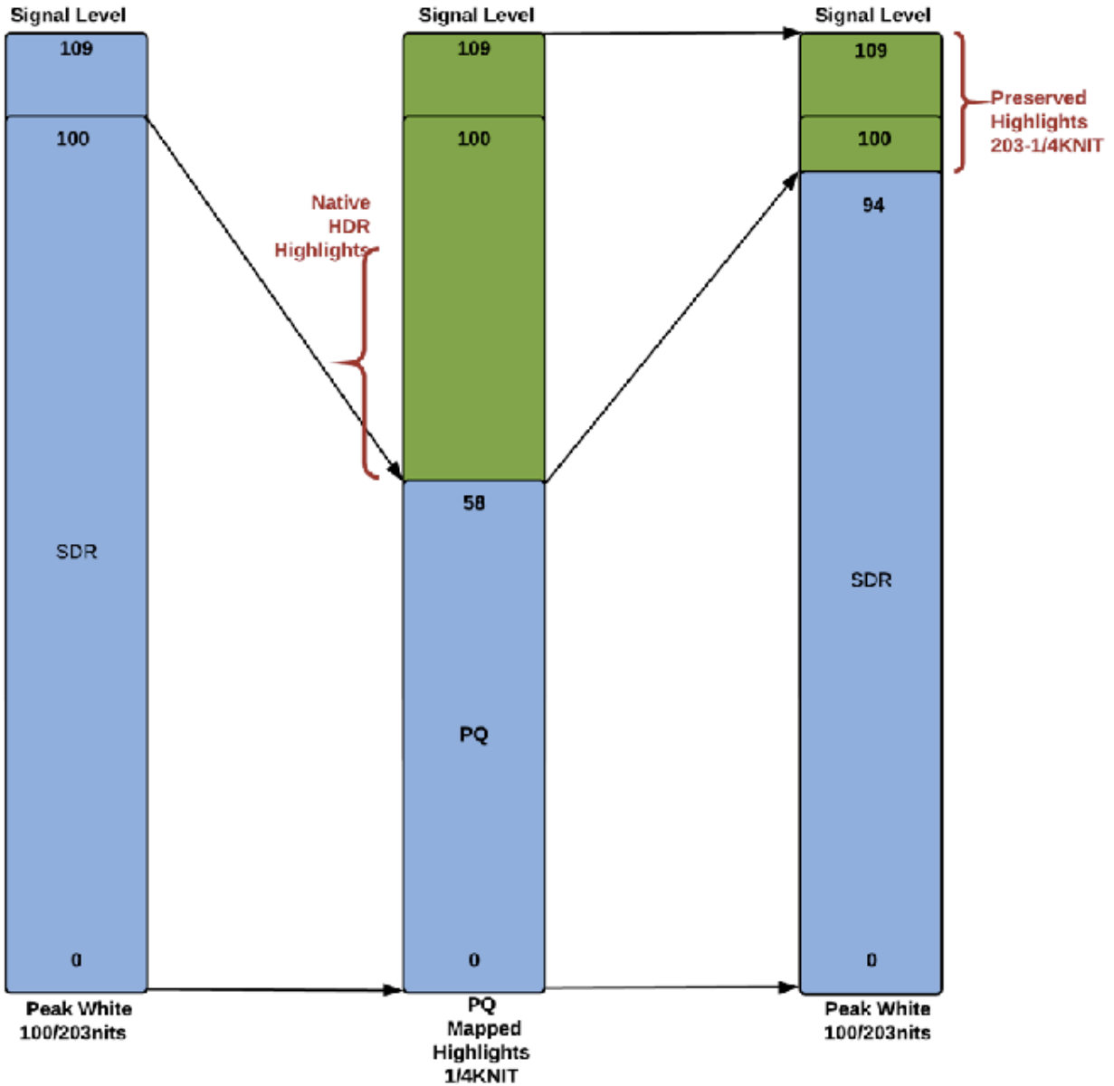
Figure 80. SDR to PQ to SDR Roundtrip Anchor Points
