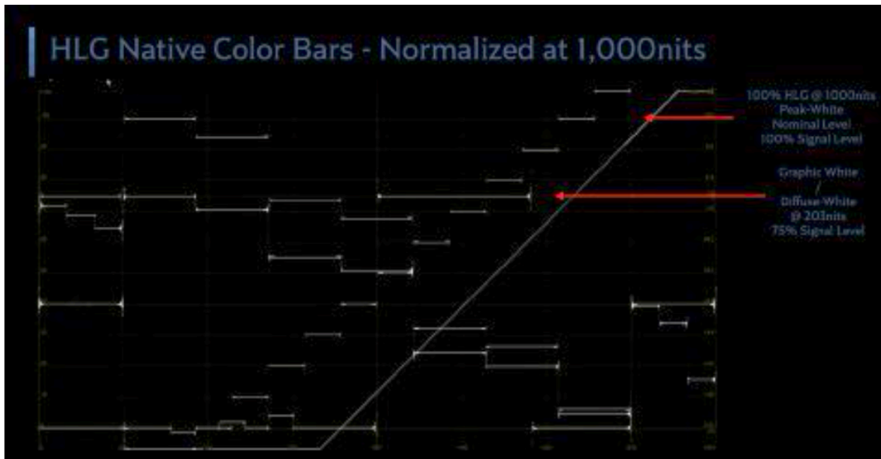
Figure 68. HDR Native Color Bars-Normalized at 1000 nits
