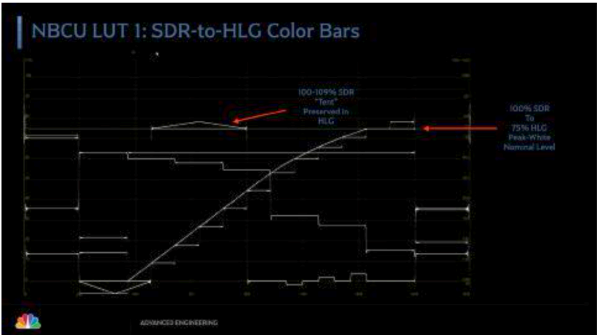
Figure 67. NBCU LUT1: SDR to HLG, SMPTE Bars with Gray 10% Ladder
