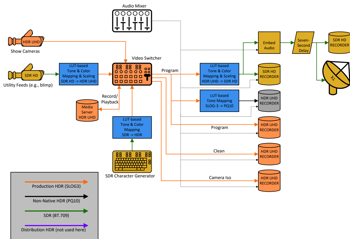
Figure 77 Amazon Major Parade Workflow
