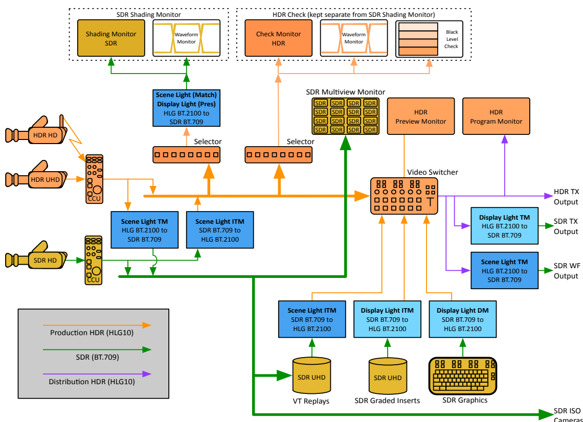
Figure 80 BBC 2019 Football Association Challenge Cup Workflow
