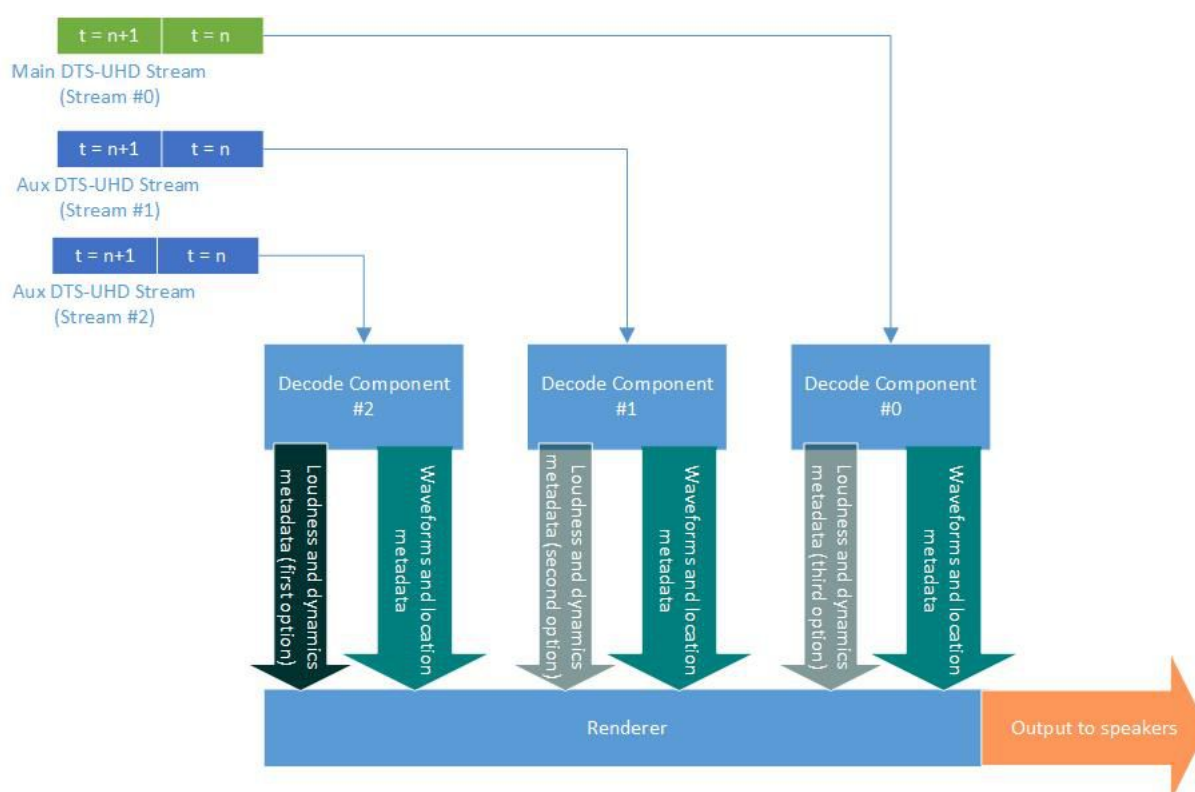
Figure 68 Example of multi-stream decoding
