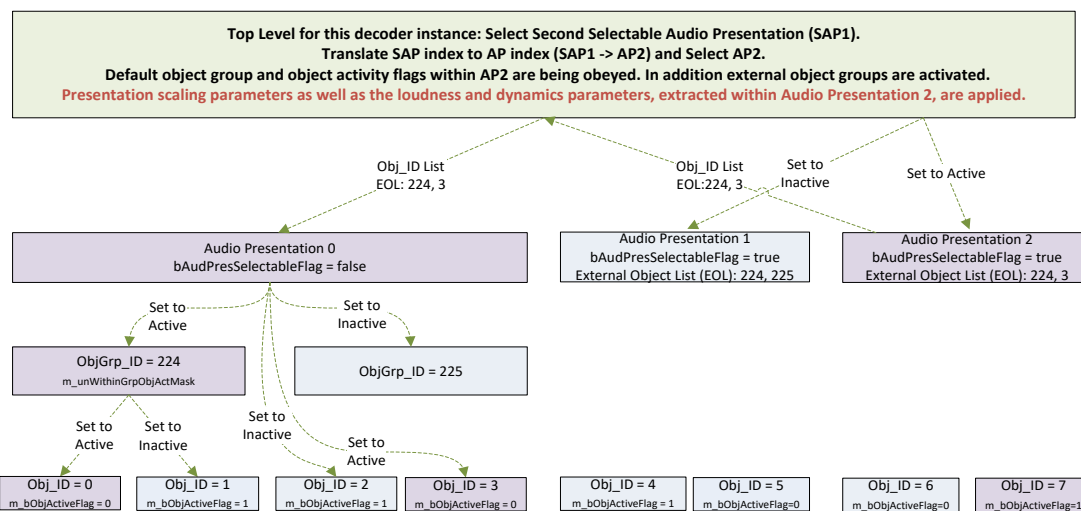
Figure 66 Example of Selecting Playback of Audio Presentation 2
