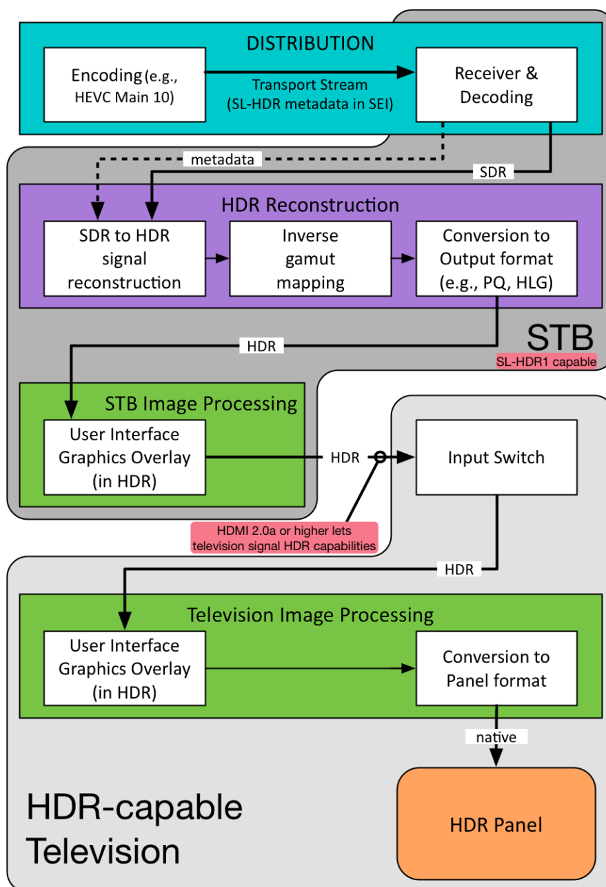
Figure 30 STB processing of SL-HDR signals for an HDR-capable television
