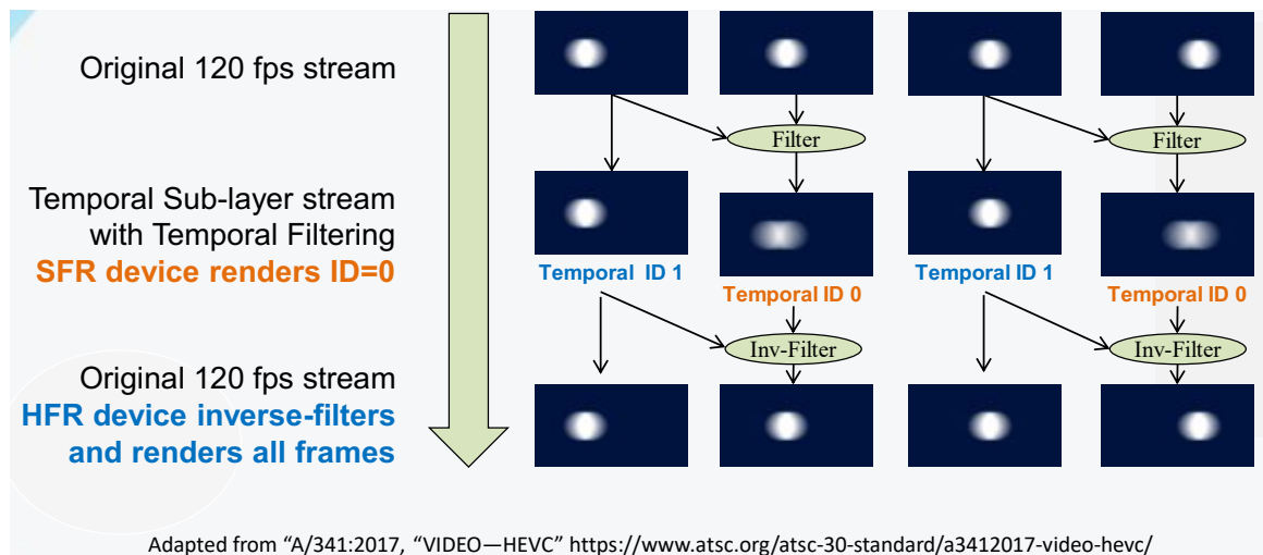
Figure 44 ATSC 3.0 temporal filtering for HFR backward compatibility
