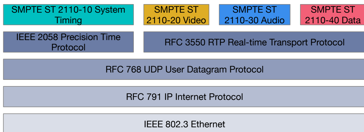
Figure 84 SMPTE ST 2110 protocol stack
