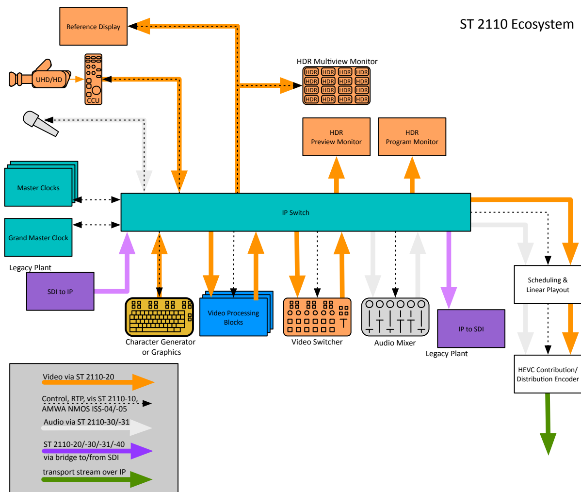
Figure 85 SMPTE ST 2110 live production workflow
