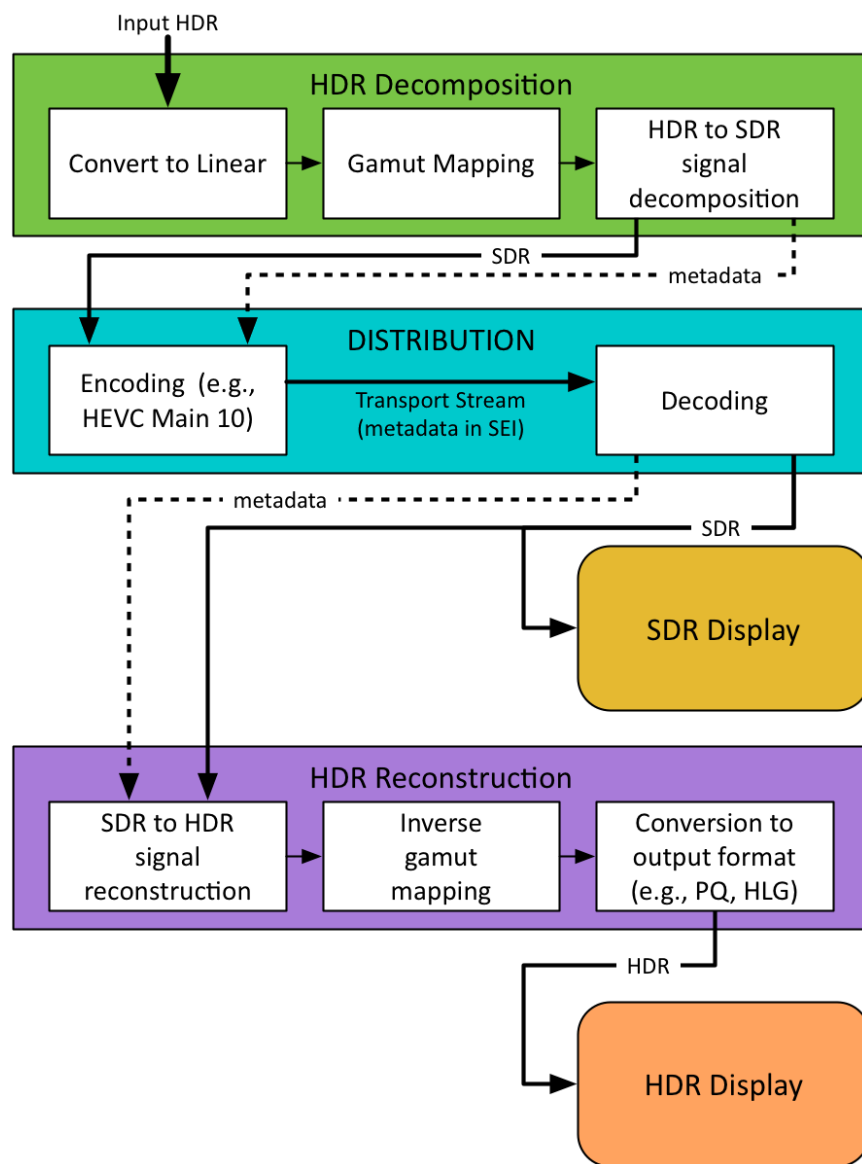
Figure 28 SL-HDR processing, distribution, reconstruction, and presentation
