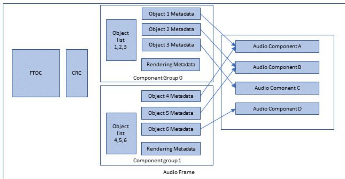
Figure 62 DTS-UHD Audio Frame Structure Example
