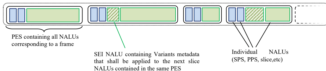
Figure 9 Transport at the Media Layer Using MPEG SEI NALUs
