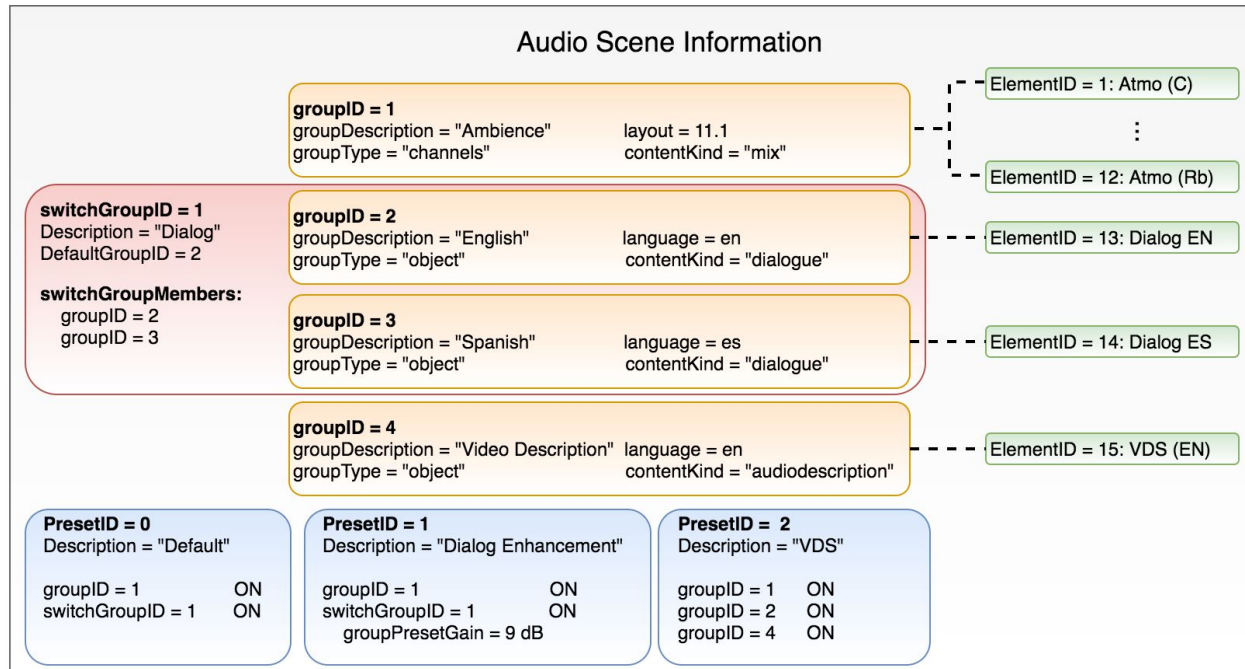
Figure 50 Example of an MPEG-H Audio Scene information
