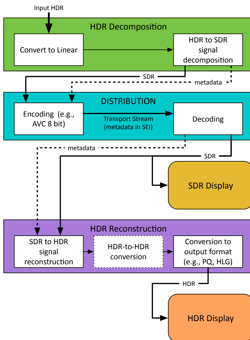
Figure 87: Signal flow for Brazil's TV 2.5
