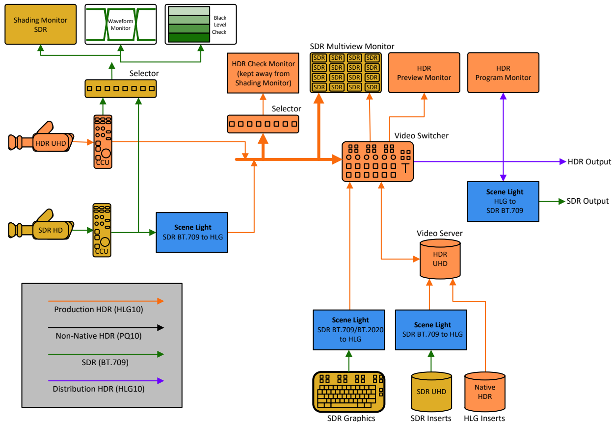
Figure 79 Sky/BBC Royal Wedding and Major Tennis Tournament Workflow
