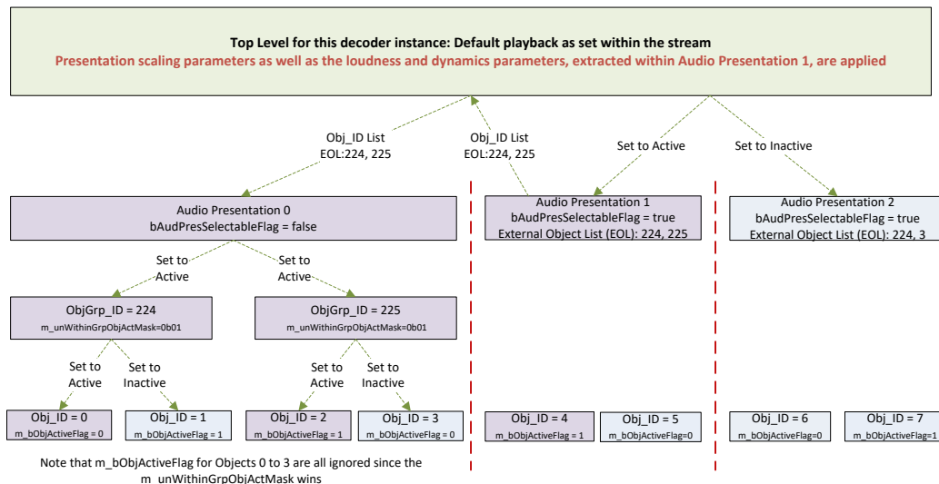
Figure 78 Playback using Default settings
