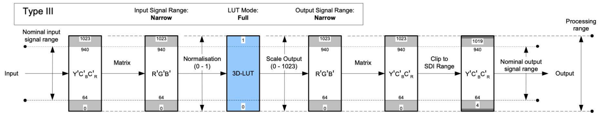
Figure 114 Type III LUT
