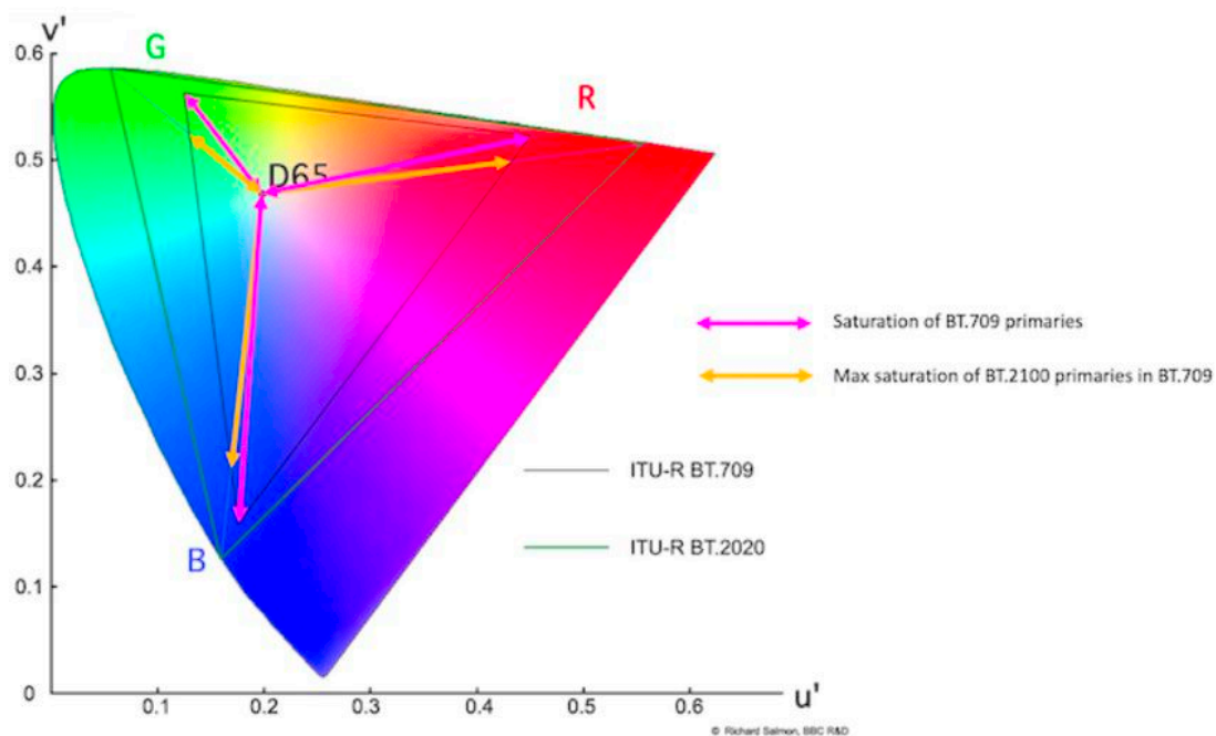
HLG-BT.2100 to SDR-BT.709 using NBCU LUT3 BT.709 Primaries and Boundaries (Sarnoff BT.2020 Yellow Brick Road)
