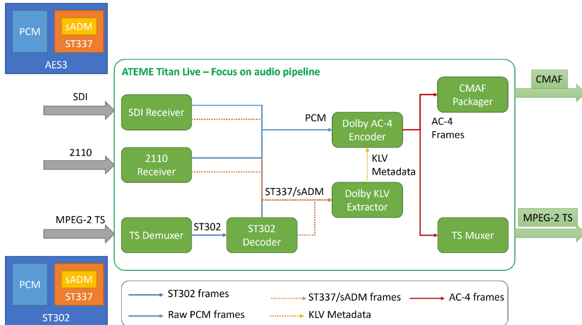
Figure 140 Encoding pipeline using an ATEME Titan Live Encoder
