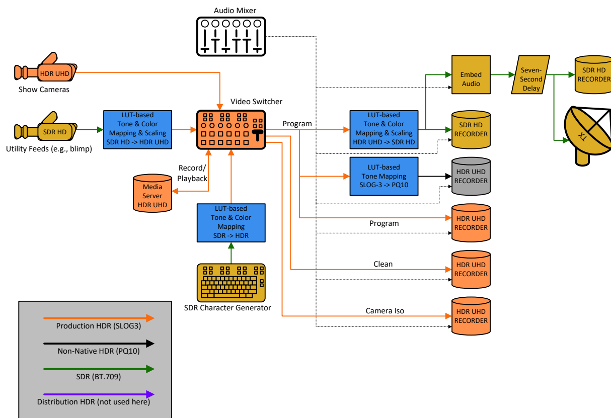
Figure 90 Amazon Major Parade Workflow
