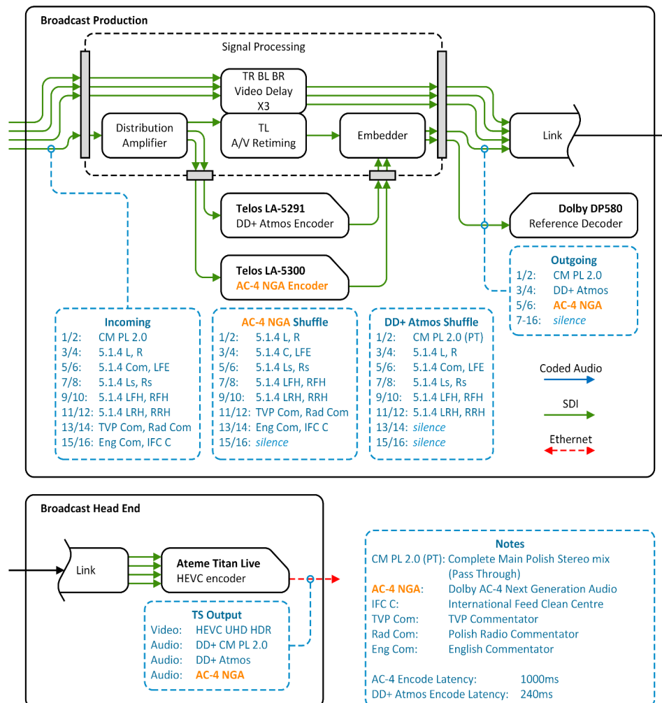
Figure 138 TVP 4K, Live EURO transmission with Atmos
