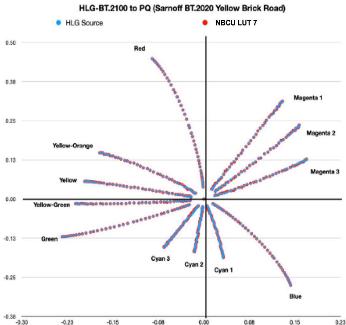
Figure 128 HLG (BT.2100) to PQ (BT.2100)
