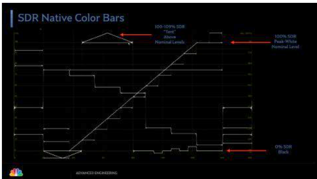
Figure 117 SDR Native SMPTE Bars with Gray 10% Ladder
