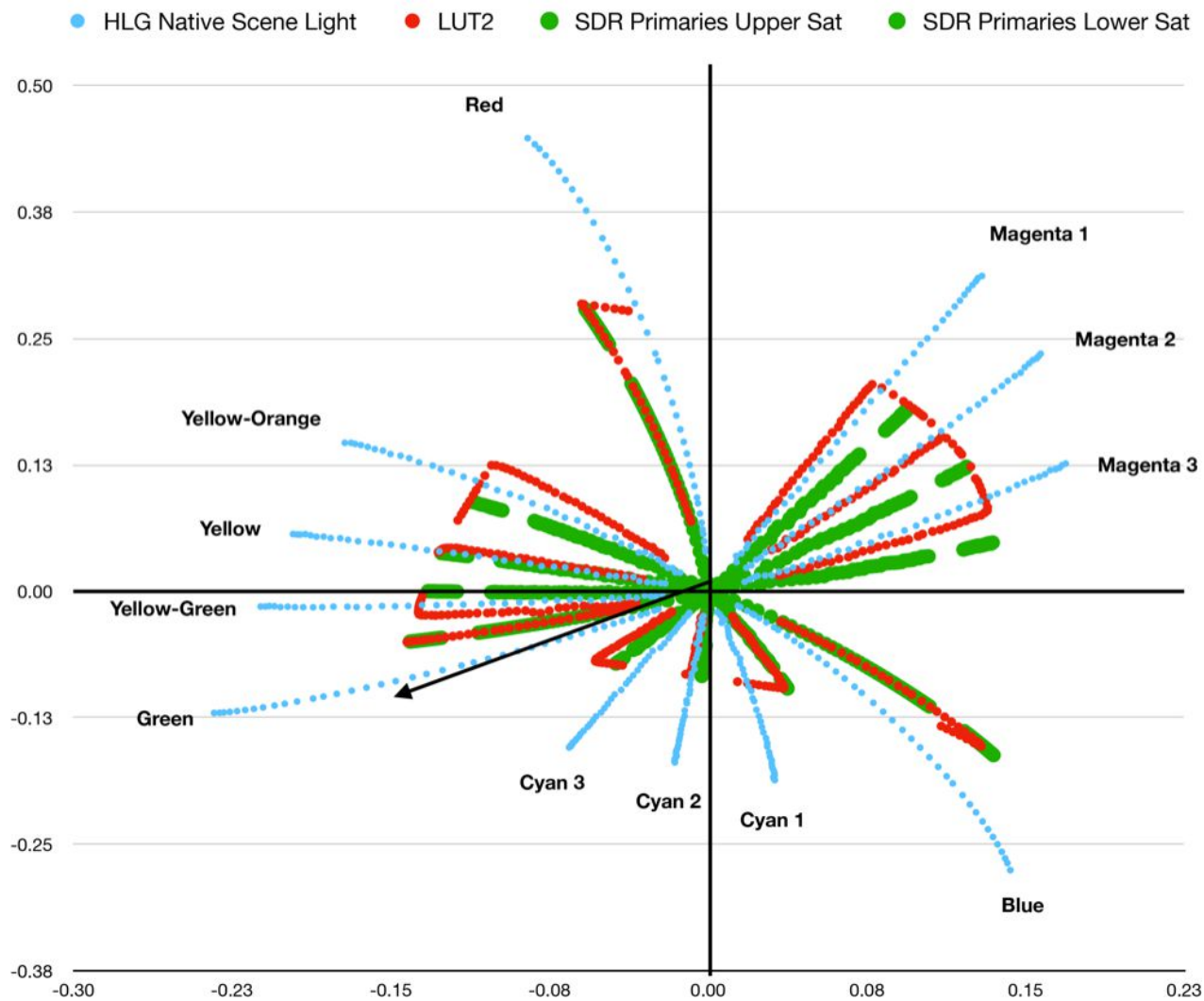
Figure 24 LUT2 Conversion from HLG to SDR
