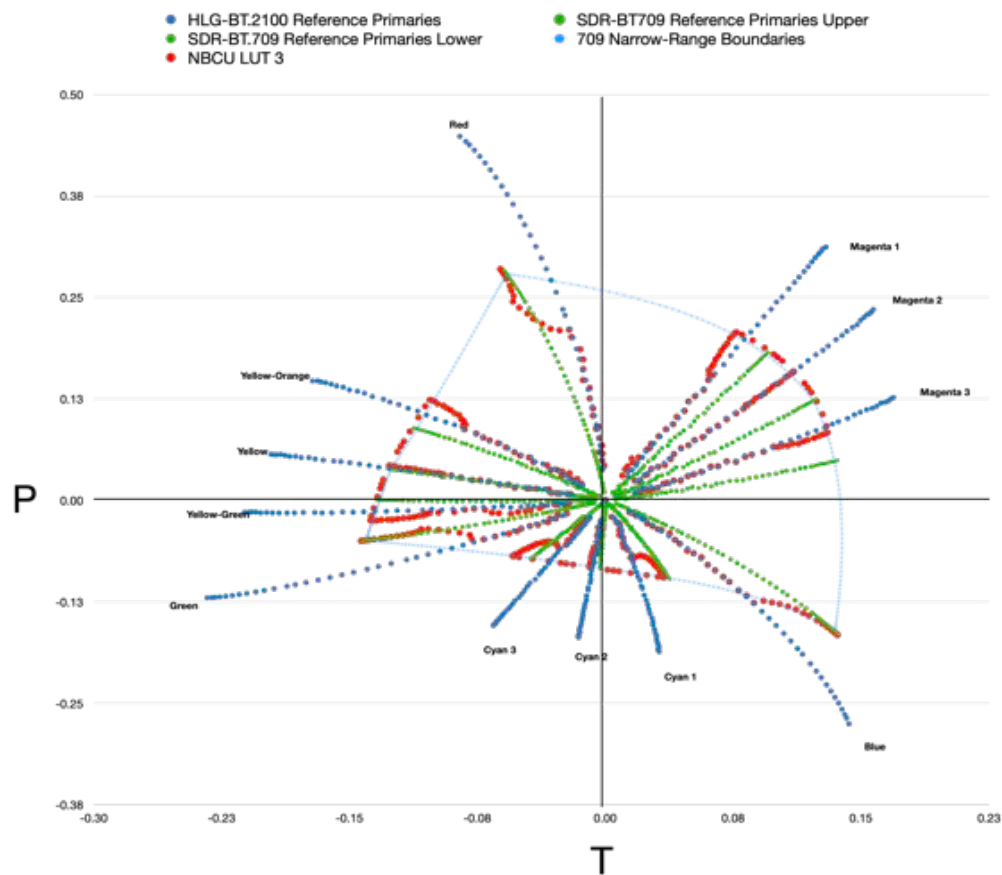
HLG-BT.2100 to SDR-BT.709 using NBCU LUT3 BT.709 Primaries and Boundaries (Sarnoff BT.2020 Yellow Brick Road)
