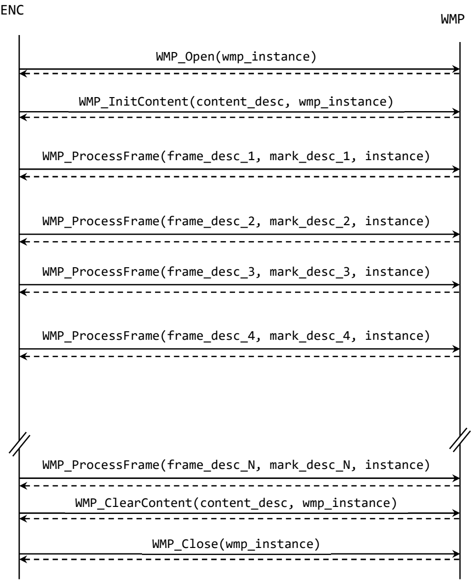
Figure 4, the function WMP_ProcessFrame() is blocking and ENC waits for WMP to end its processing before the next call of WMP_ProcessFrame(). Note that, in this flow, the data in the returned mark_description may correspond to a video frame provided in a previous call in frame_description. This delay is expressed using the structure delay_description returned by the function WMP_InitContent().
